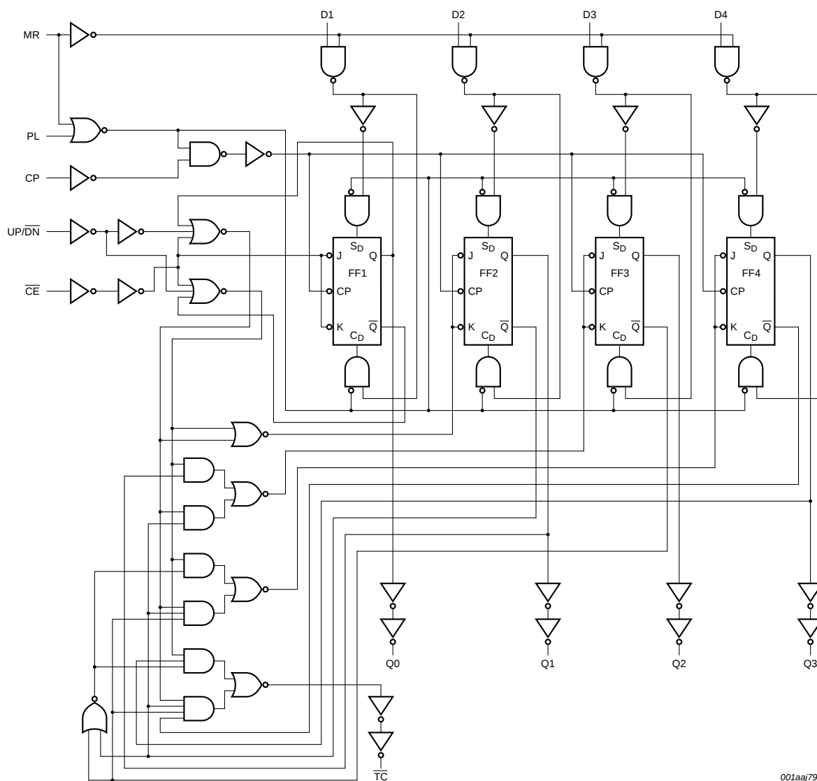
Fig 2. Logic diagram
